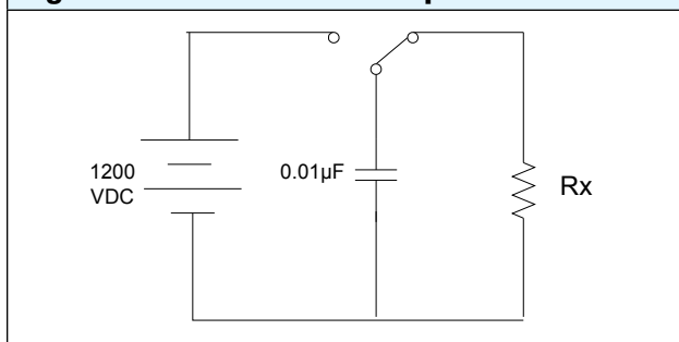
Figure 7—Pulse Test Description
