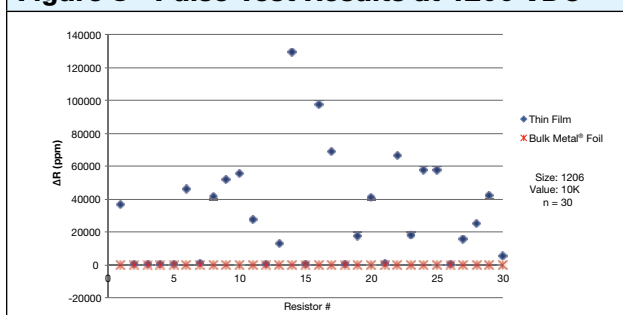
Figure 8—Pulse Test Results at 1200 VDC*
