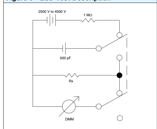
Figure 9—ESD Test Description
